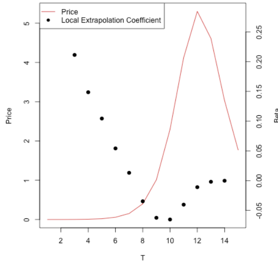
Figure 9. Time-Varying Extrapolation
